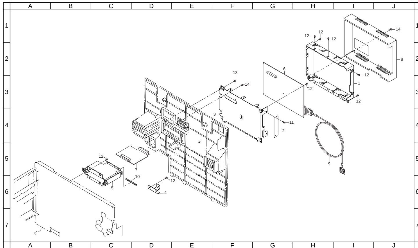
FIG. 1 PRINTER KIT
